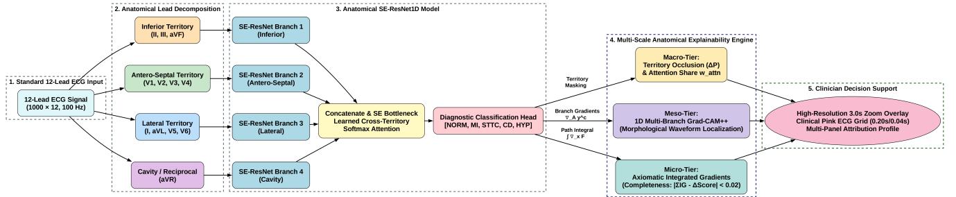
Figure 4: Architectural overview of the Hierarchical Multi-Scale Anatomical Explainability (XAI) Framework. Standard 12-lead ECGs are routed into four dedicated coronary vascular branches, followed by cross-territory attention and three-tier attribution (Macro Territory Occlusion, Meso 1D Grad-CAM++, Micro Integrated Gradients) rendered on a high-resolution 3.0s clinical pink grid.
